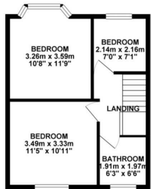
1ST FLOOR 35.96 sq. m. ( 387.08 sq. ft. )
